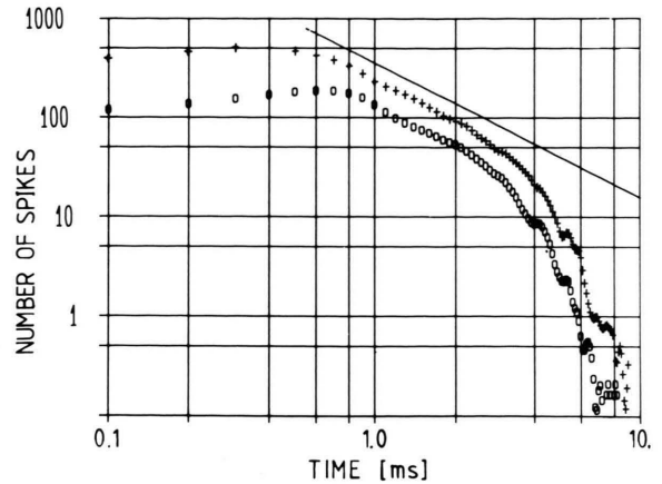
Fig. 2. Distribution of time intervals between current spikes obtained at the bias voltages V_0 = 349 mV (circles) and V_0 = 370 mV (crosses). In the range 0.6–6 ms the curves can be approximated by a solid straight line of slope -1.33 .
